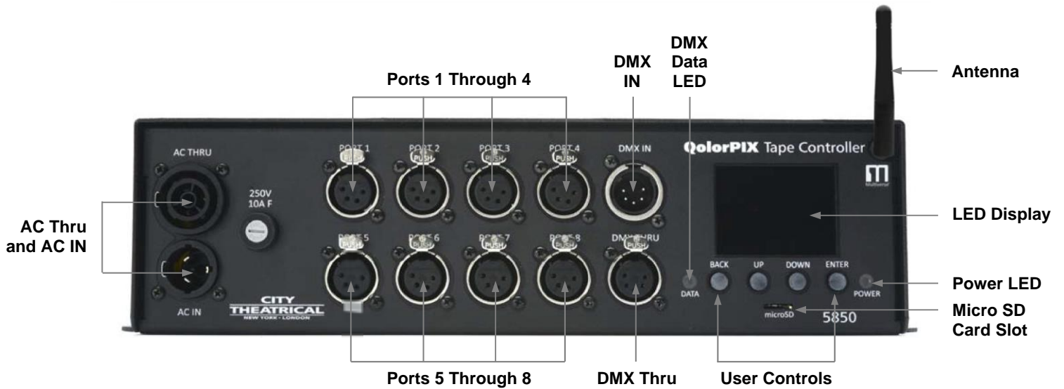
Figure 6: Face Panel
